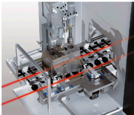
Pre-control unit
