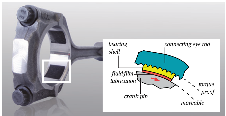
Structuring on the large connecting rod eye
