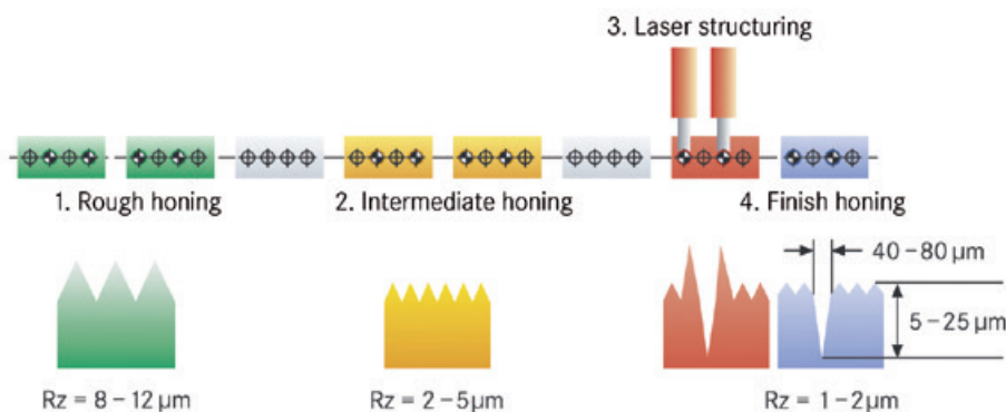
Process sequence for the laser structuring of cylinder bores
